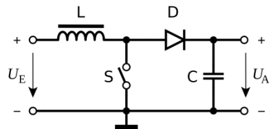
Boost-Converter, Step Up
