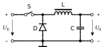
Buck Converter, Step down
