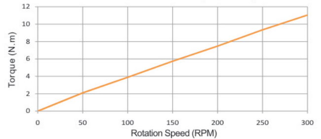
Speed-Torque Curve
