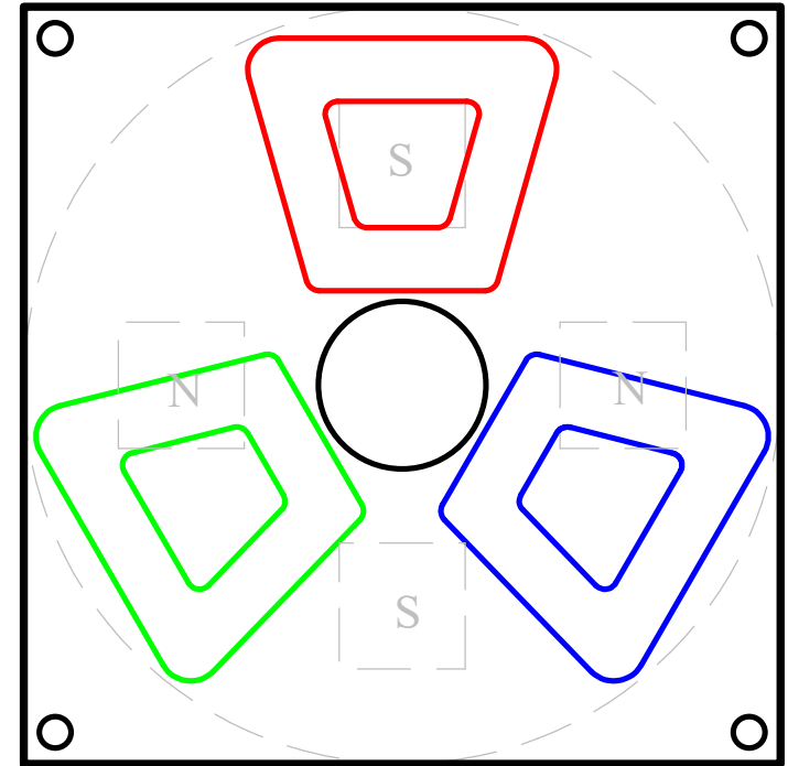
Stator
